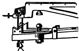
FIG. 4.—Becker's Balance. End of Beam.
