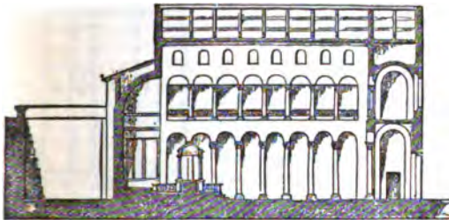
FIG. 12.—Section of Basilica of St Agnes at Roma.
