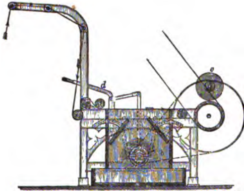
FIG. 11.—Damping-Machine.
