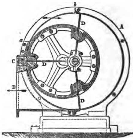
FIG. 5.—Section of an American Blowing-Machine.
