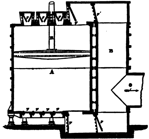
FIG. 3.—SECTION OF CYLINDER OF BLOWING ENGINE.
