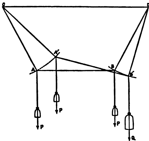
FIG. 1.—Diagram Illustrating Chain Balance.
