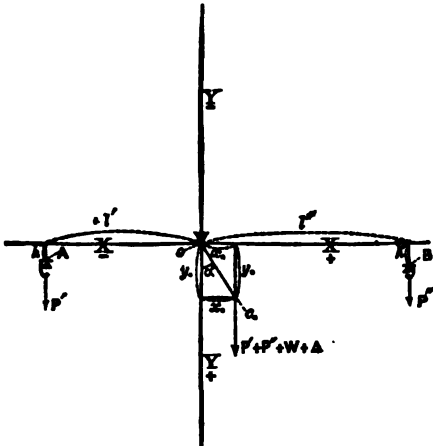
FIG. 7.—Diagram illustrating theory of Precision Balance.
