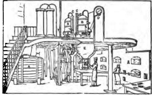
FIG. 3.—Dauglish Apparatus—double set.
