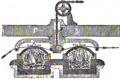
FIG. 4.—Section of Singe-Stove.
