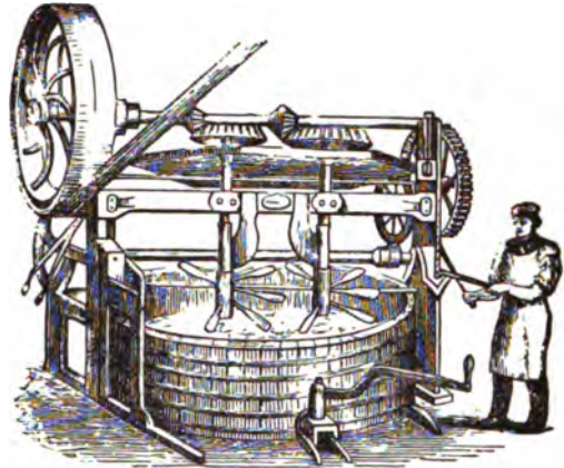
FIG. 7.—Patent Vertical Mixer.
