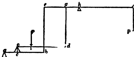
FIG. 9.—Decimal Balance.
