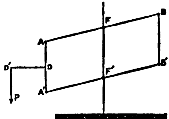
FIG. 8.—Roberval's Balance.
