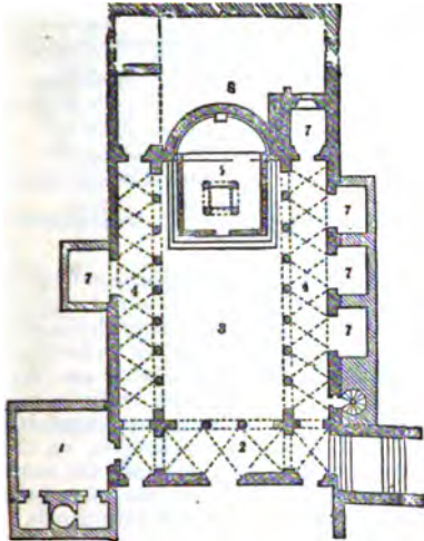
FIG. 11.—Ground-Plan of Basilica of St Agnes at Roma.
