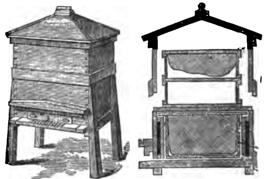
FIG. 5.—The Cheshire Frame Hive. FIG. 6.—Section of Cheshire Hive.
