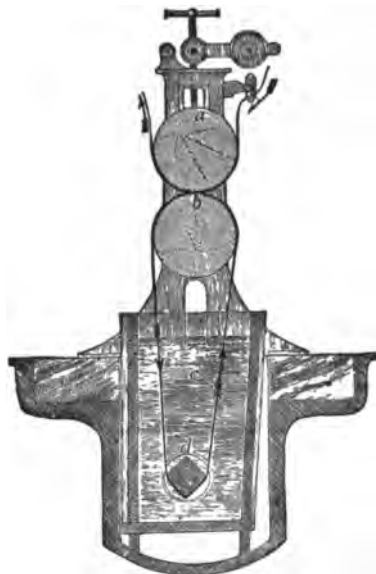
FIG. 9.—Section of Washing-Machine.
