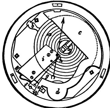
FIG. 5.—Aneroid Barometer.
