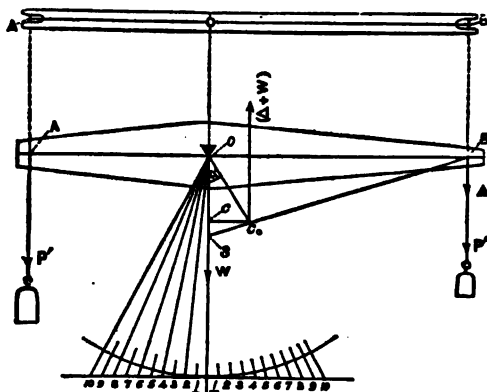
FIG. 2.—Diagram illustrating the theory of the Lever Balance.
