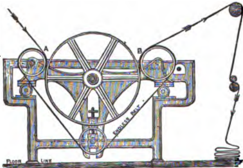
FIG. 12.—Elevation of Belt-Stretching Machine.
