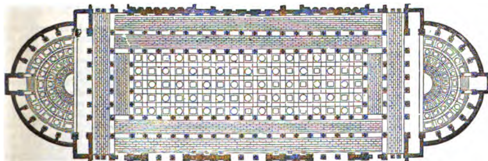
FIG. 3.—Ground-Plan of Trajan's Basilica ( Basilica Ulpia ).
