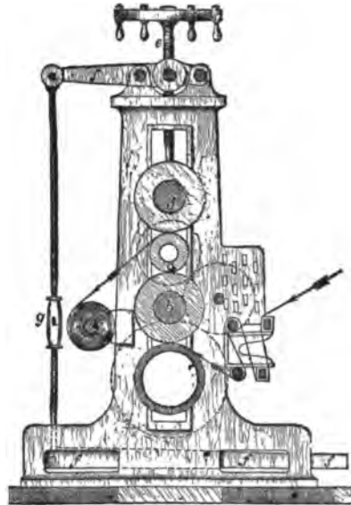
FIG. 17.—Section of Calender.
