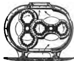
FIG. 6.—Rotary Blower.
