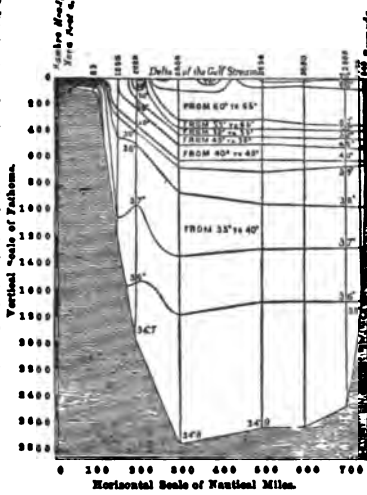
FIG. 6.—Section from Bermuda to Halifax.
